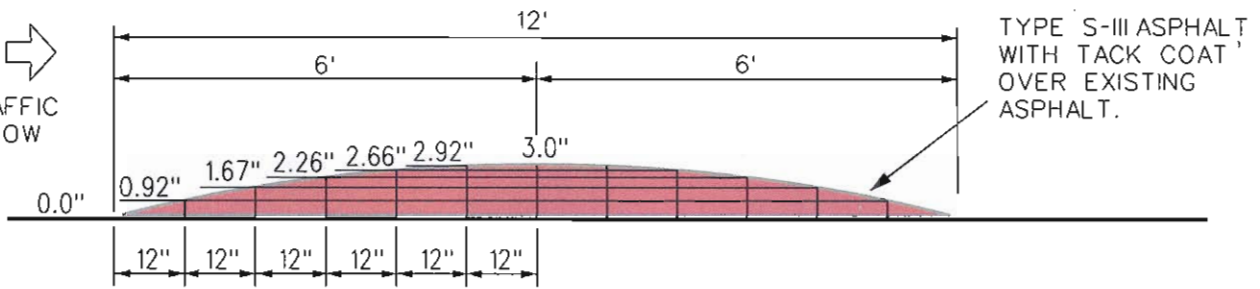
DRIVING PROFILE
