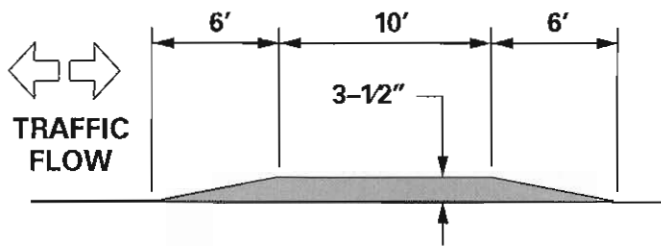
DRIVING PROFILE
