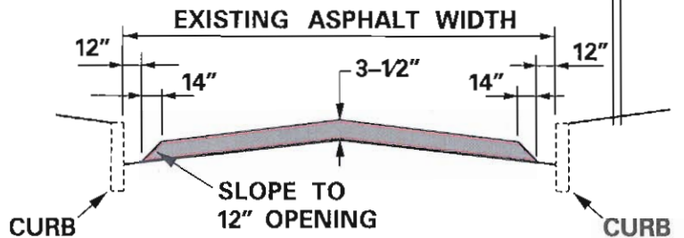
TYPICAL SECTION
